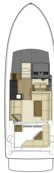
SUNROOM/COCKPIT LAYOUT
