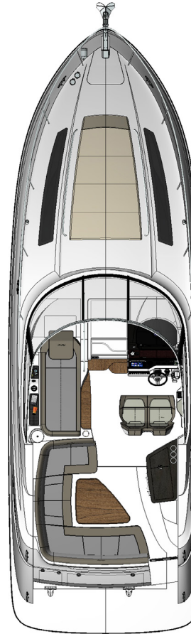
COCKPIT LAYOUT
