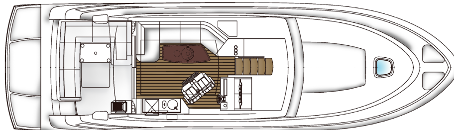
COCKPIT/SUNROOM LAYOUT
