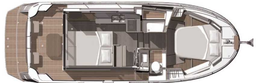
LOWER DECK 1 Cabin version | Version 1 cabine
