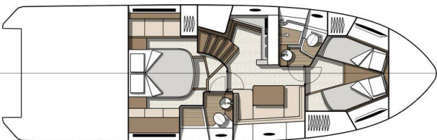
2 cabins layout
